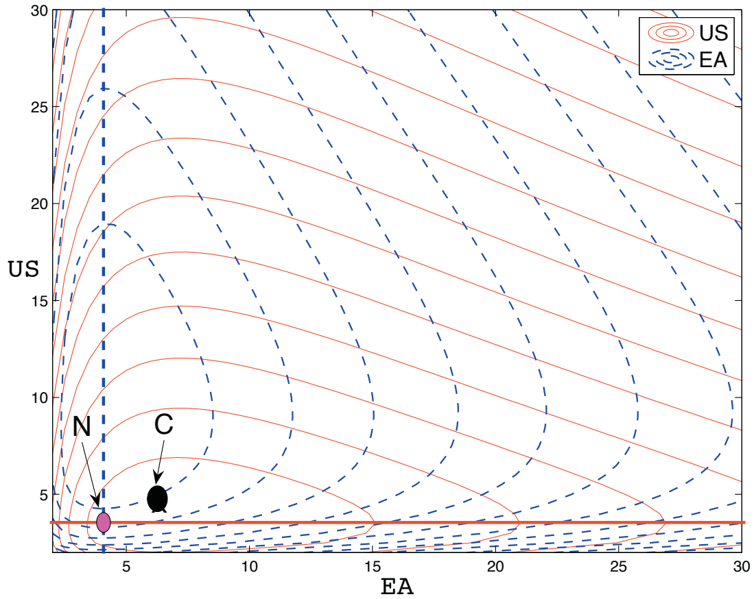
Figure 3: Nash and cooperative equilibria under inertial interest rate rules reacting to wage inflation only.
