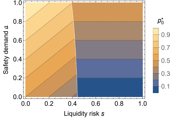
Figure 8: Equilibrium price for combinations of liquidity and safety shocks. The figure shows a contour plot of the equilibrium price p_0^* as a function of liquidity risk s and safety demand a . Parameters: v = 1.2 , b = 1 , c = 1 .
