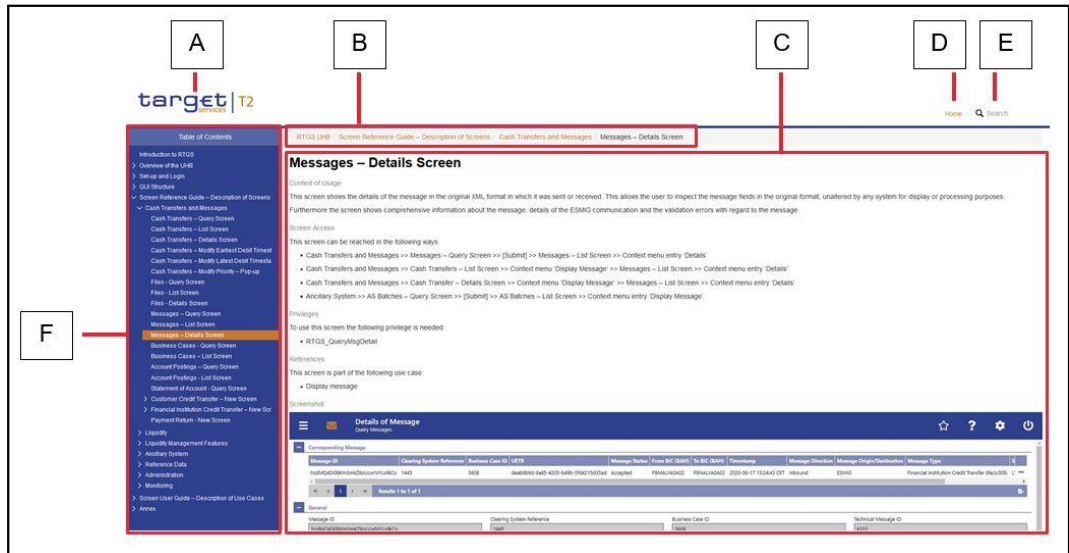
Figure 75 - Online Help
